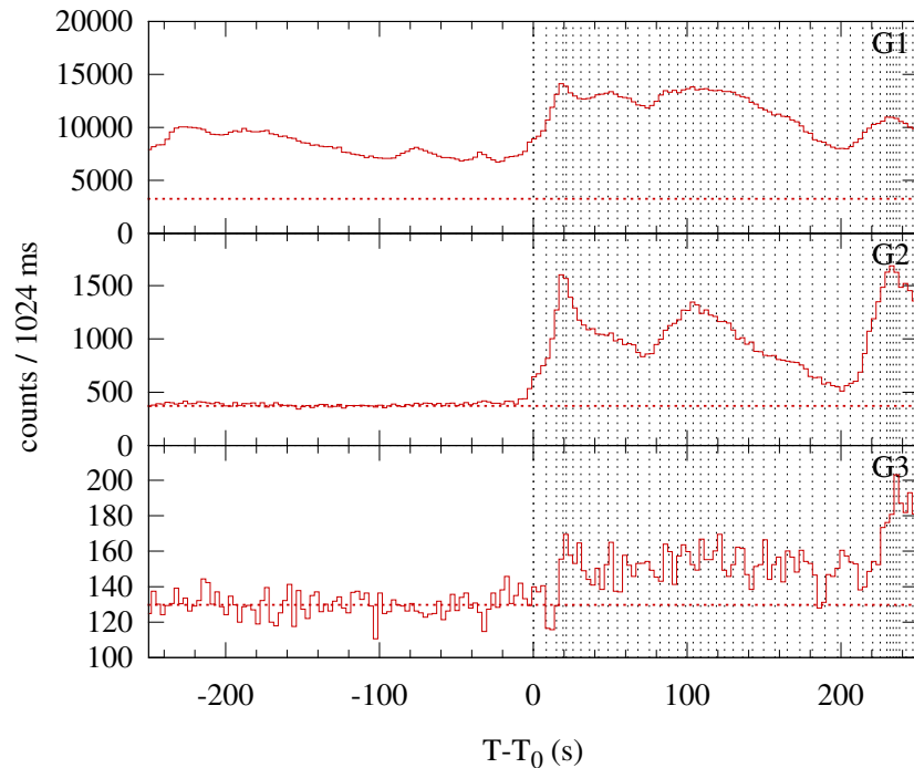
Konus-WIND S2 SOL2013-05-13T02:08 (X1.7) T 0 = 7696.811 s UT (02:08:16.811)
