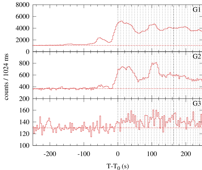
Konus-WIND S2 SOL2013-05-13T15:52 (X2.8) T_0 = 57170.166 s UT (15:52:50.166)
