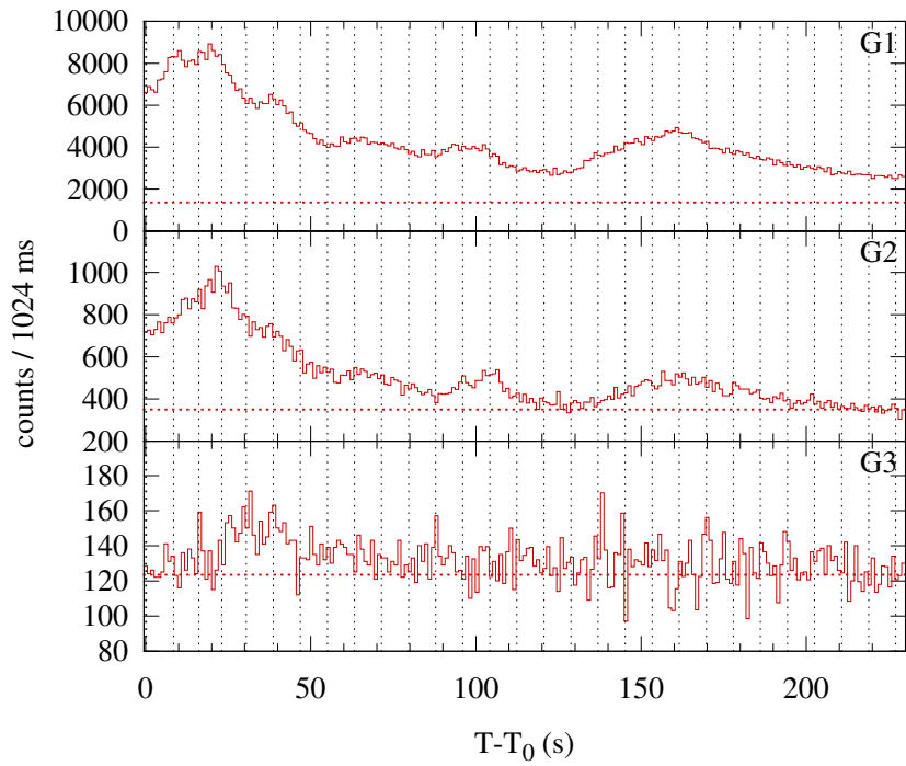
Konus-WIND S2 SOL2013-06-07T22:43 (M5.9) T_0 = 81783.340 s UT (22:43:03.340)
