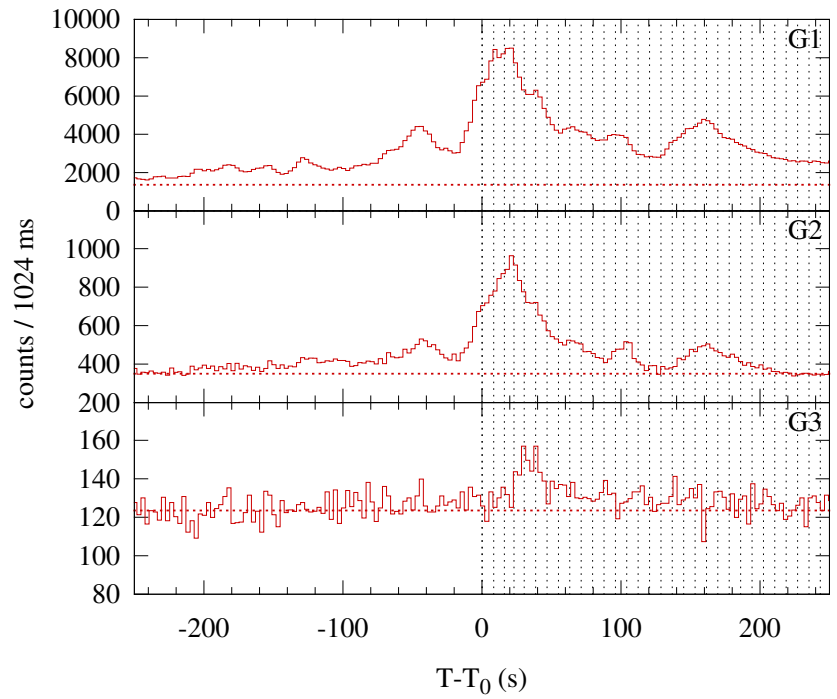
Konus-WIND S2 SOL2013-06-07T22:43 (M5.9) T_0 = 81783.340 s UT (22:43:03.340)
