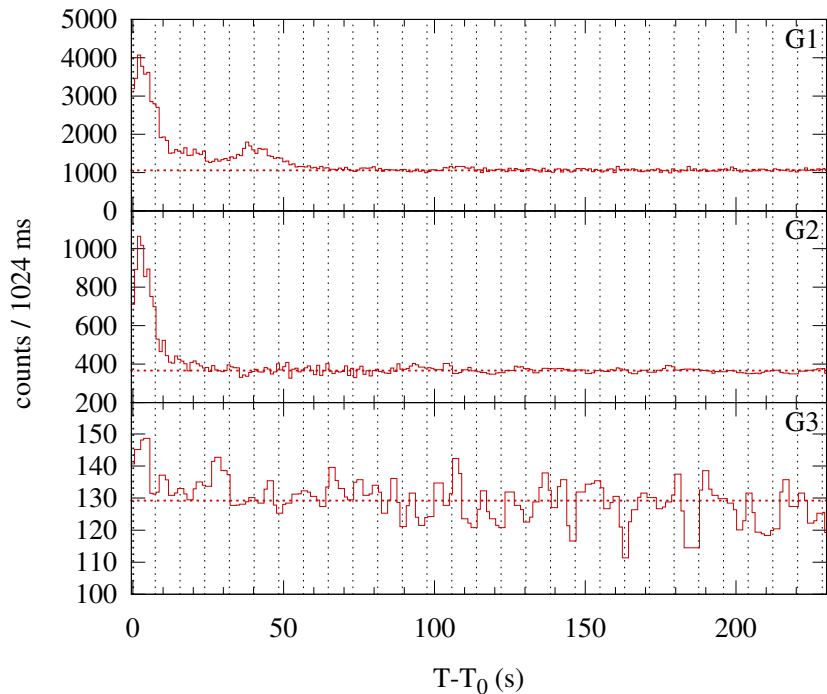
Konus-WIND S2 SOL2013-10-18T10:52 (C4.7) T_0 = 39162.378 s UT (10:52:42.378)
