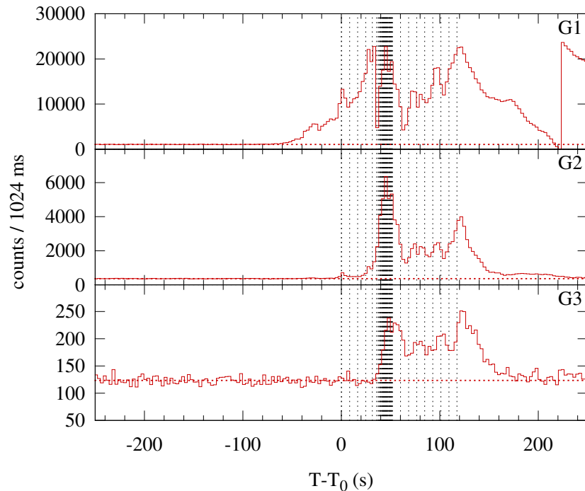
Konus-WIND S2 SOL2013-10-25T07:57 (X1.7) T_0 = 28643.377 s UT (07:57:23.377)
