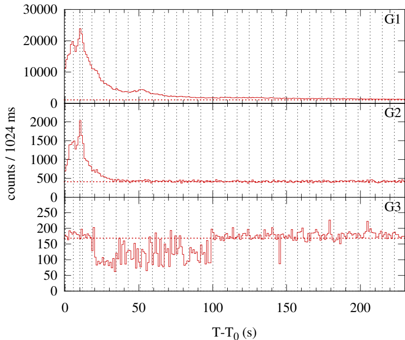
Konus-WIND S2 SOL2013-10-25T20:56 (M1.9) T 0 = 75404.68 s UT (20:56:44.68)
