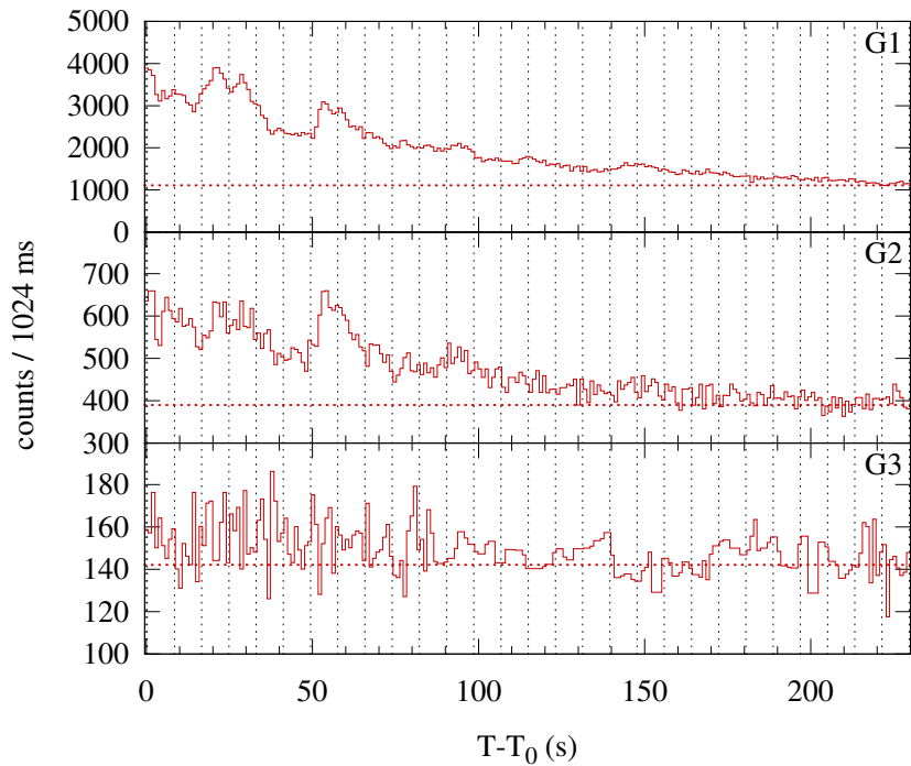
Konus-WIND S2 SOL2013-10-26T19:24 (M3.1) T_0 = 69851.650 s UT (19:24:11.650)
