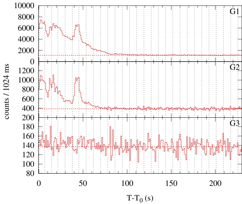
Konus-WIND S2 SOL2013-10-27T17:50 (C9.1) T 0 = 64251.617 s UT (17:50:51.617)
