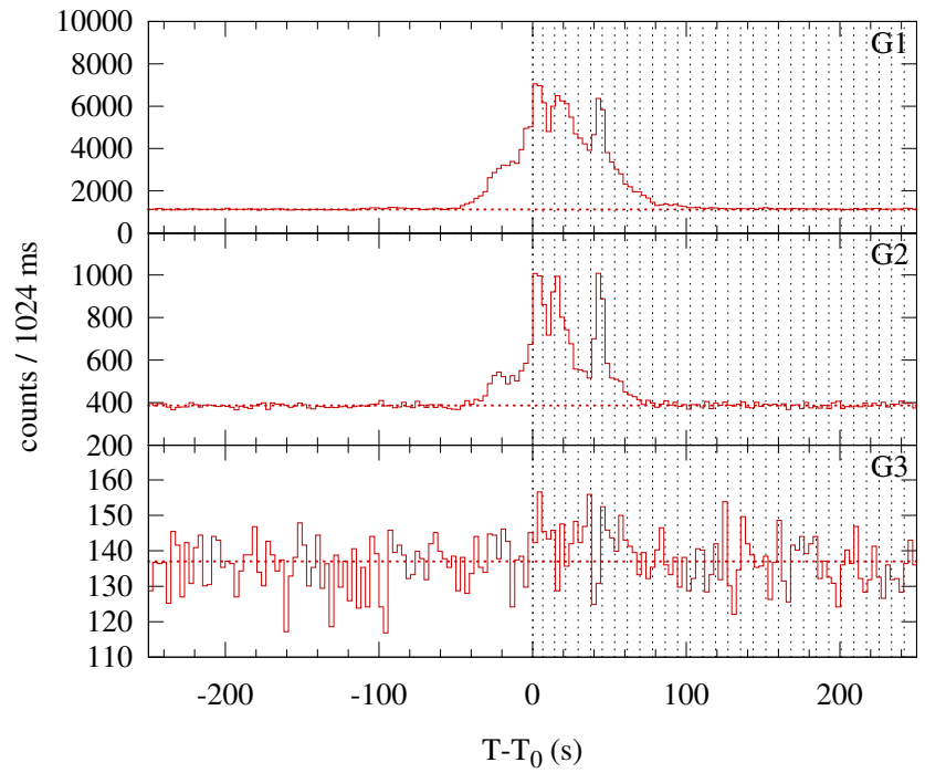
Konus-WIND S2 SOL2013-10-27T17:50 (C9.1) T 0 = 64251.617 s UT (17:50:51.617)
