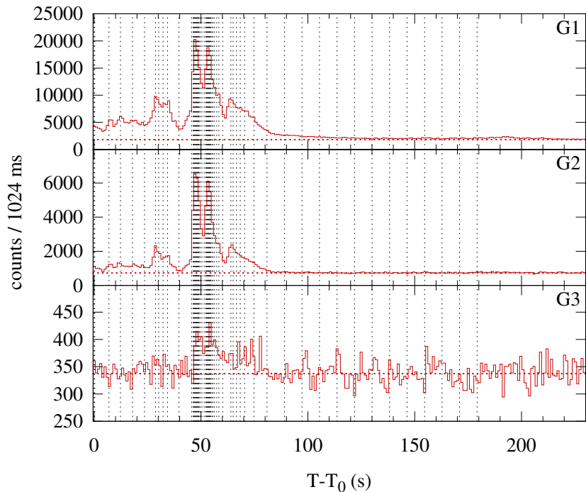
Konus-WIND S2 SOL2013-10-28T20:53 (M1.5) T 0 = 75234.930 s UT (20:53:54.930)
