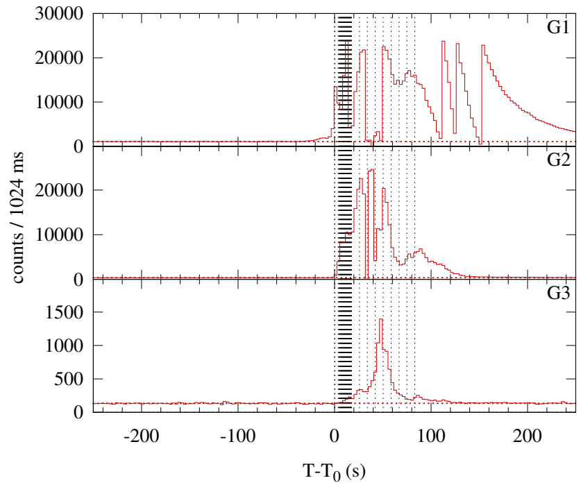
Konus-WIND S2 SOL2013-11-05T22:10 (X3.3) T 0 = 79848.194 s UT (22:10:48.194)
