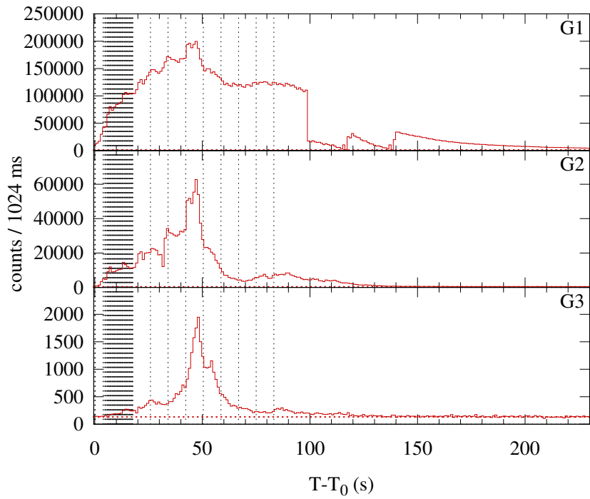
Konus-WIND S2 SOL2013-11-05T22:10 (X3.3) T 0 = 79848.194 s UT (22:10:48.194)
