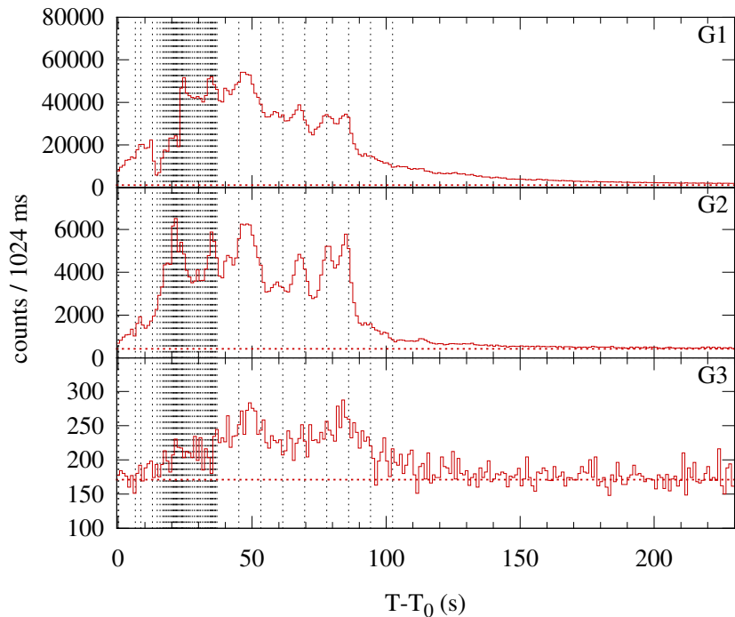
Konus-WIND S2 SOL2013-11-08T04:23 (X1.1) T 0 = 15821.76 s UT (04:23:41.76)
