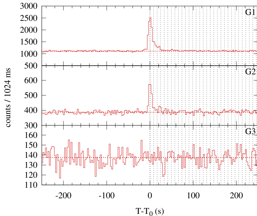
Konus-WIND S2 SOL2013-11-12T06:22 (C3.2) T 0 = 22961.74 s UT (06:22:41.74)
