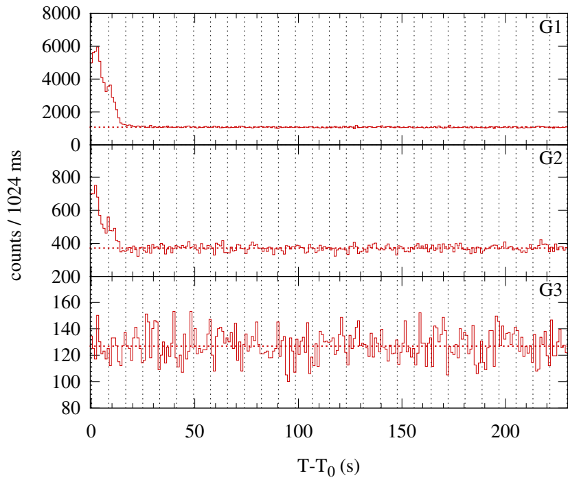
Konus-WIND S2 SOL2013-11-14T06:45 (C3.5) T_0 = 24330.974 s UT (06:45:30.974)
