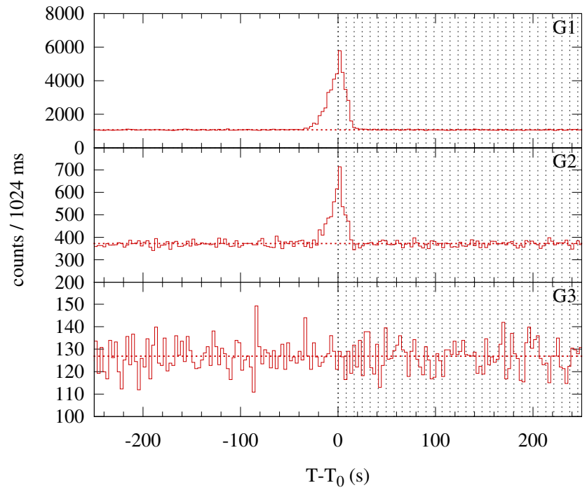
Konus-WIND S2 SOL2013-11-14T06:45 (C3.5) T_0 = 24330.974 s UT (06:45:30.974)
