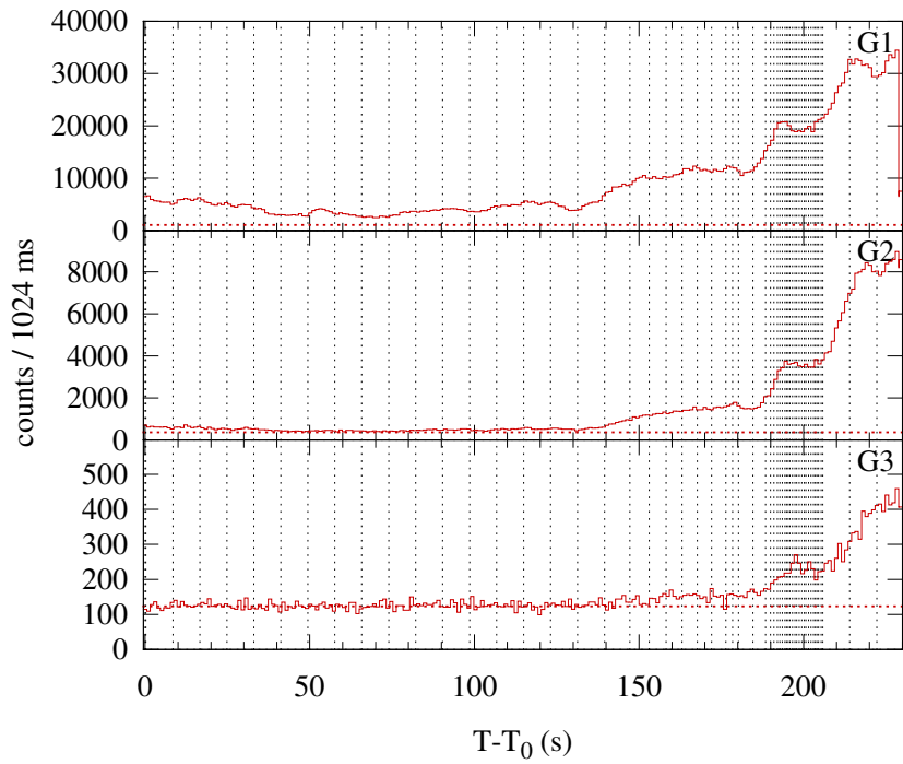
Konus-WIND S2 SOL2013-11-19T10:18 (X1.0) T_0 = 37090.924 s UT (10:18:10.924)
