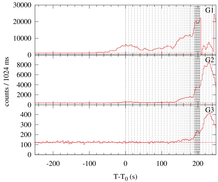
Konus-WIND S2 SOL2013-11-19T10:18 (X1.0) T_0 = 37090.924 s UT (10:18:10.924)
