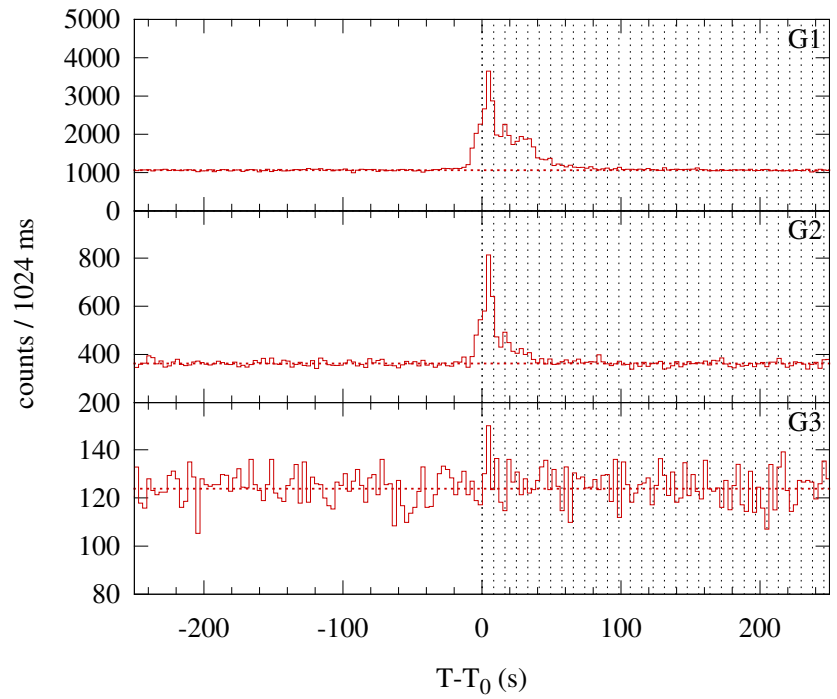
Konus-WIND S2 SOL2014-01-28T05:27 (C9.2) T_0 = 19631.135 s UT (05:27:11.135)
