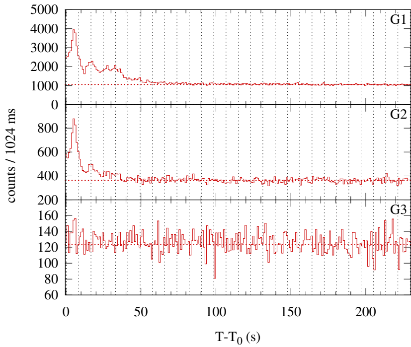
Konus-WIND S2 SOL2014-01-28T05:27 (C9.2) T_0 = 19631.135 s UT (05:27:11.135)
