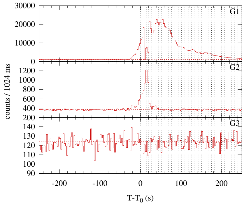
Konus-WIND S2 SOL2014-02-04T03:58 (M5.2) T 0 = 14300.116 s UT (03:58:20.116)
