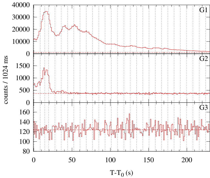
Konus-WIND S2 SOL2014-02-04T03:58 (M5.2) T 0 = 14300.116 s UT (03:58:20.116)
