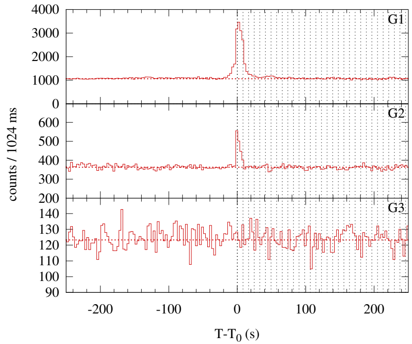
Konus-WIND S2 SOL2014-02-04T15:30 (M1.5) T_0 = 55815.976 s UT (15:30:15.976)
