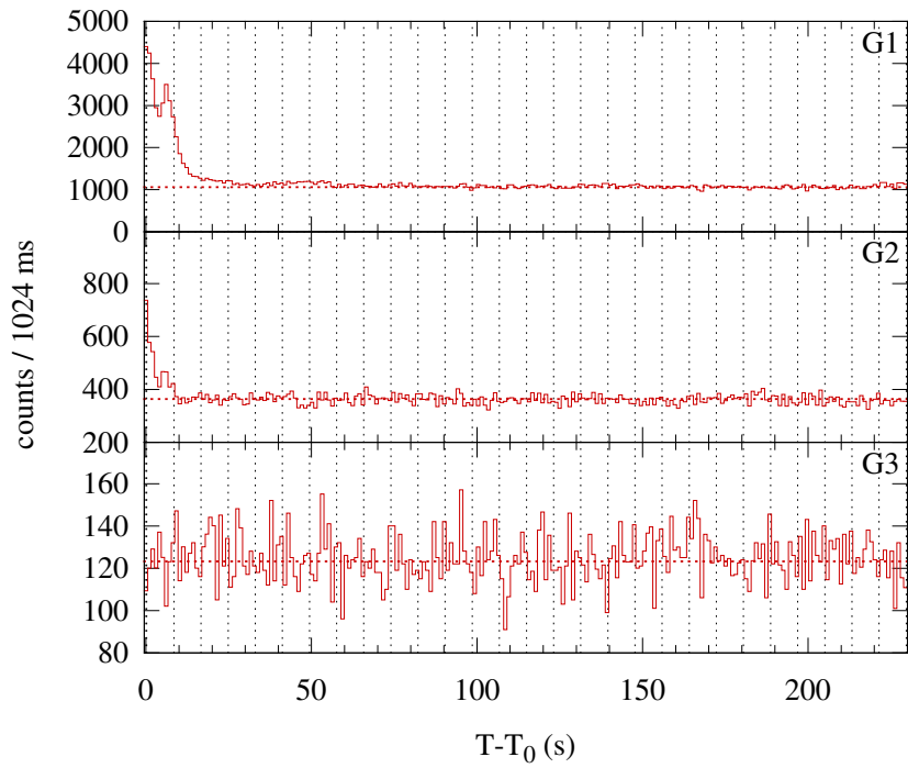
Konus-WIND S2 SOL2014-02-04T15:30 (M1.5) T_0 = 55815.976 s UT (15:30:15.976)
