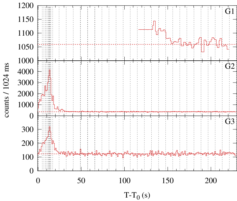
Konus-WIND S2 SOL2014-02-07T10:27 (M1.9) T_0 = 37676.74 s UT (10:27:56.74)
