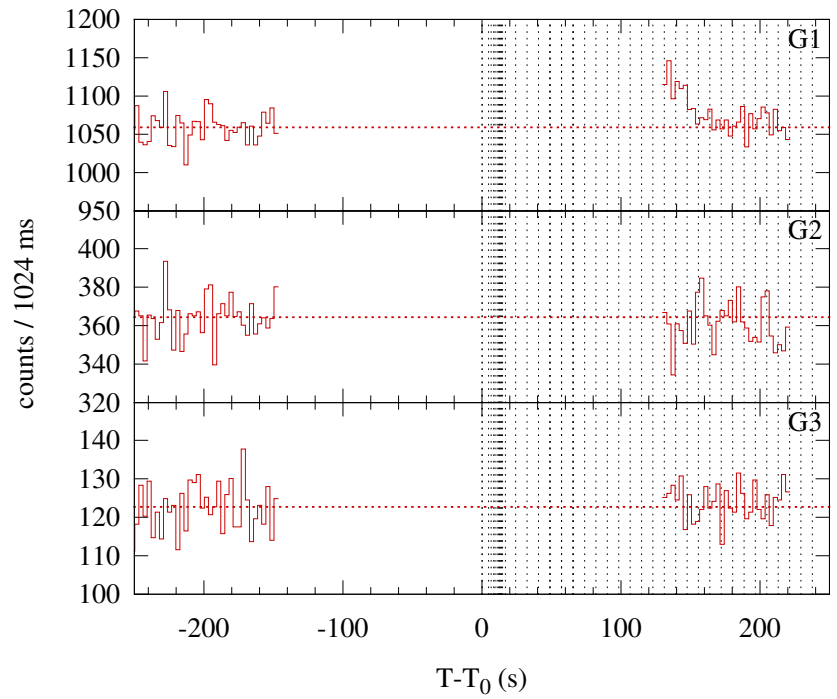
Konus-WIND S2 SOL2014-02-07T10:27 (M1.9) T_0 = 37676.74 s UT (10:27:56.74)
