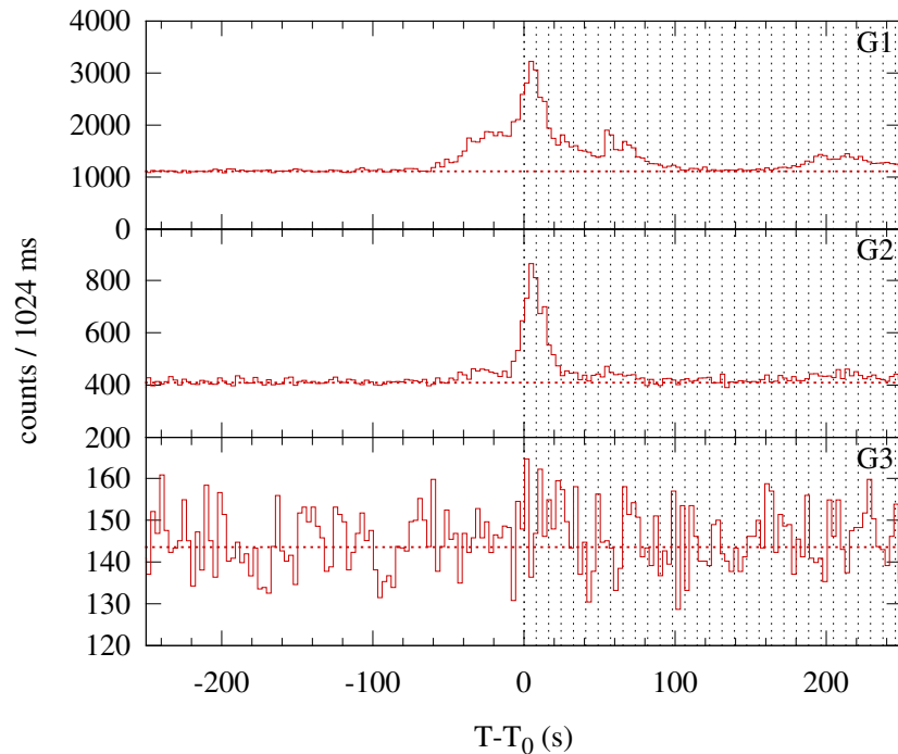
Konus-WIND S2 SOL2014-02-14T16:36 (M1.0) T 0 = 59772.172 s UT (16:36:12.172)
