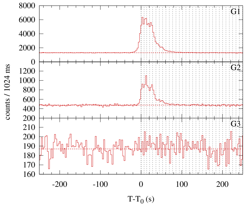
Konus-WIND S2 SOL2014-03-03T15:57 (M1.2) T 0 = 57441.63 s UT (15:57:21.63)
