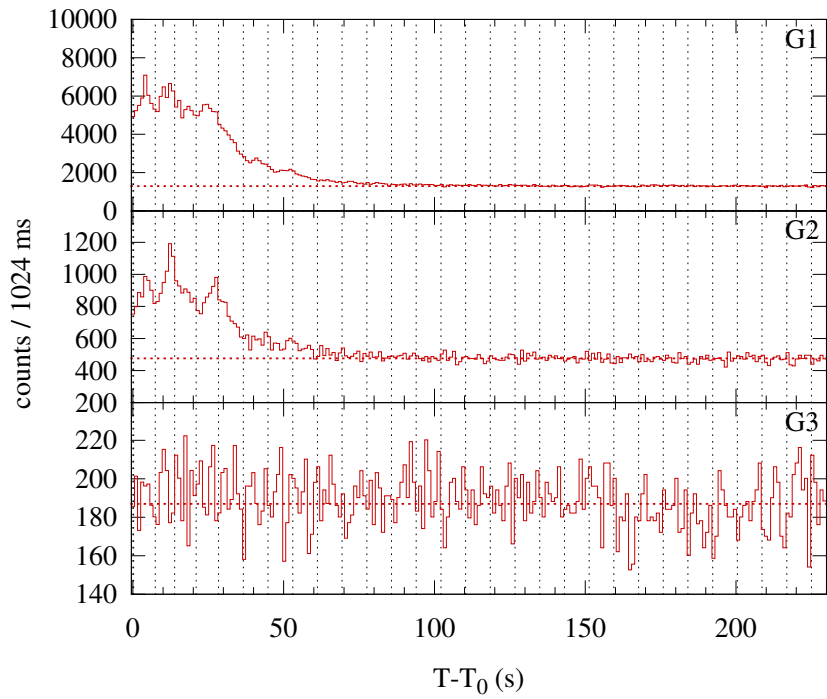
Konus-WIND S2 SOL2014-03-03T15:57 (M1.2) T 0 = 57441.63 s UT (15:57:21.63)
