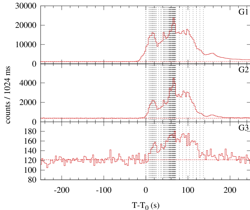
Konus-WIND S2 SOL2014-03-29T17:45 (X1.0) T_0 = 63919.106 s UT (17:45:19.106)
