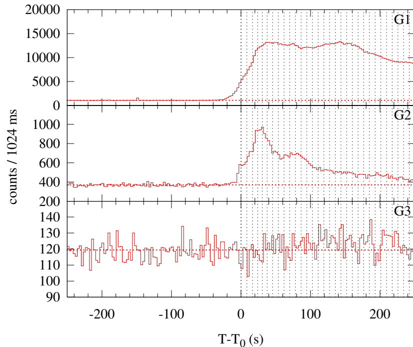
Konus-WIND S2 SOL2014-04-25T00:20 (X1.3) T_0 = 1210.166 s UT (00:20:10.166)
