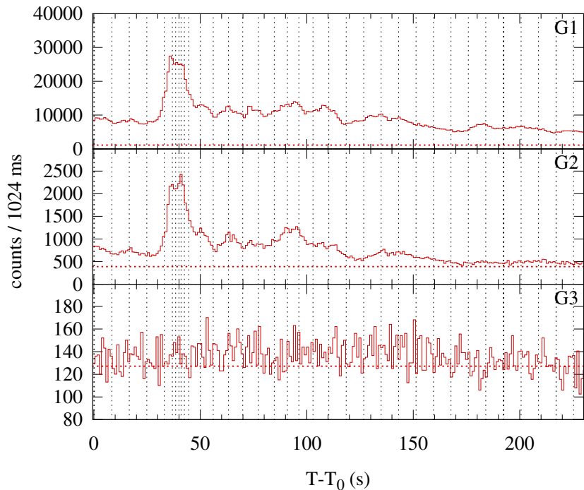
Konus-WIND S2 SOL2014-05-08T10:01 (M5.2) T 0 = 36096.97 s UT (10:01:36.97)
