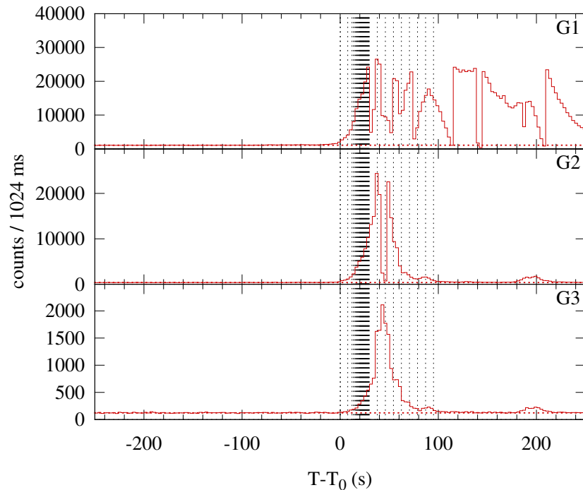
Konus-WIND S2 SOL2014-06-10T11:39 (X2.2) T 0 = 41951.280 s UT (11:39:11.280)
