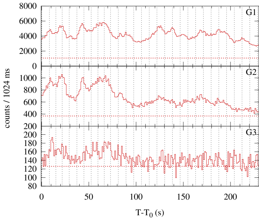
Konus-WIND S2 SOL2014-08-24T12:10 (M5.9) T_0 = 43800.607 s UT (12:10:00.607)
