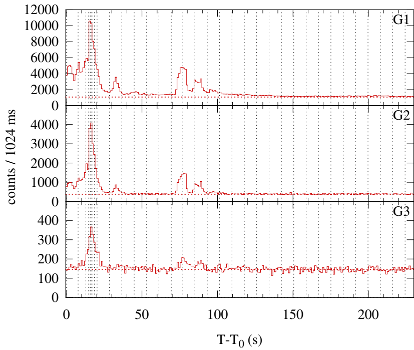
Konus-WIND S2 SOL2014-09-18T08:39 (M1.2) T_0 = 31187.949 s UT (08:39:47.949)
