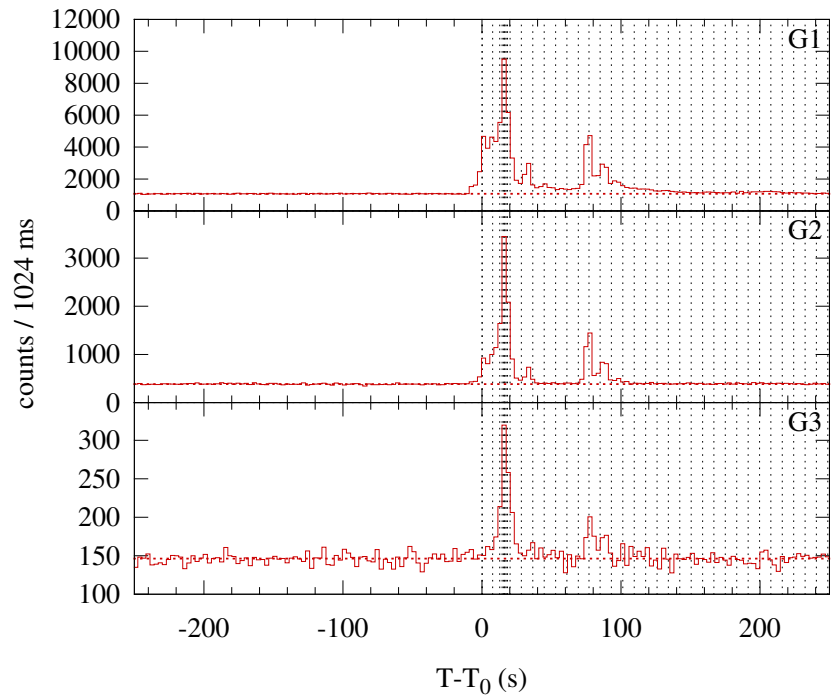
Konus-WIND S2 SOL2014-09-18T08:39 (M1.2) T_0 = 31187.949 s UT (08:39:47.949)
