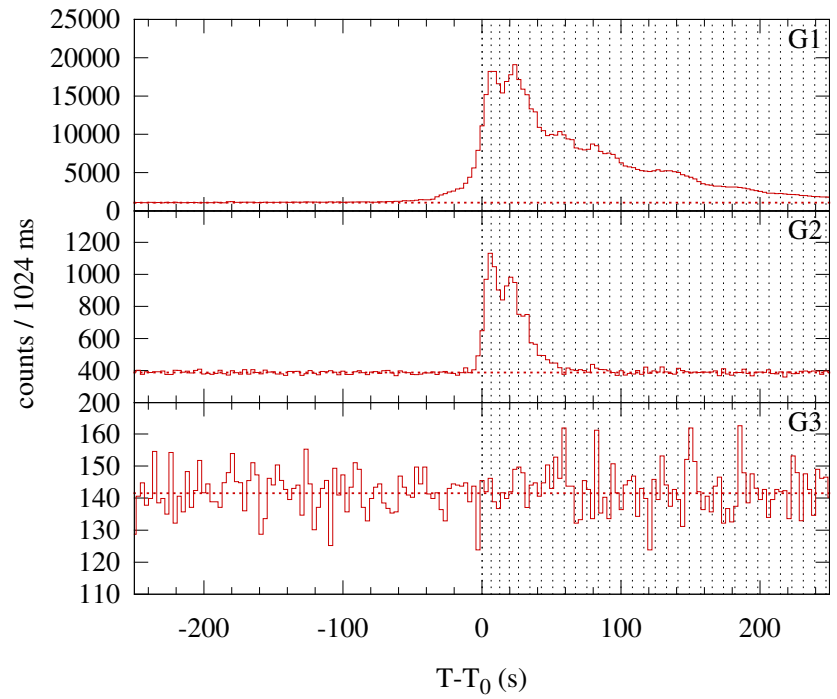
Konus-WIND S2 SOL2014-10-20T09:05 (M3.9) T 0 = 32738.985 s UT (09:05:38.985)
