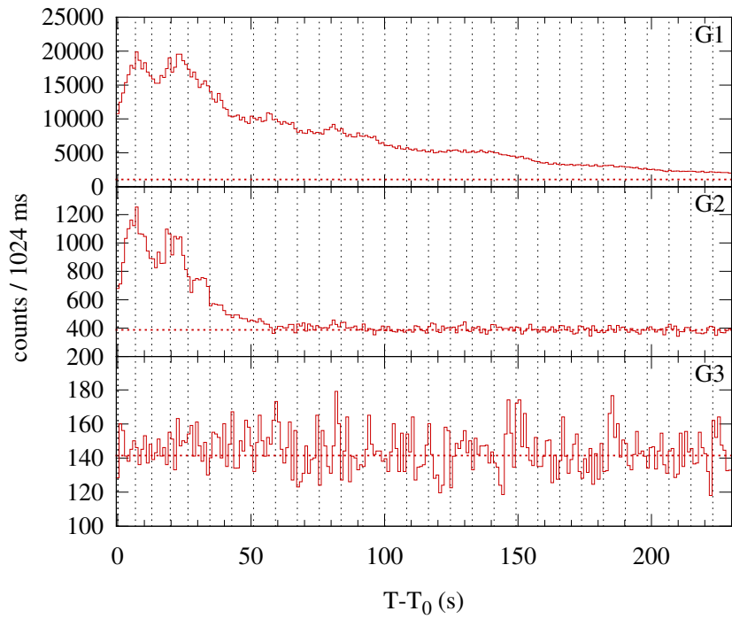
Konus-WIND S2 SOL2014-10-20T09:05 (M3.9) T 0 = 32738.985 s UT (09:05:38.985)
