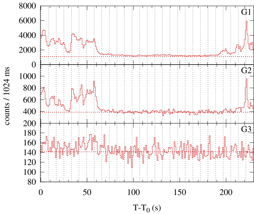
Konus-WIND S2 SOL2014-10-20T18:57 (M1.4) T 0 = 68272.493 s UT (18:57:52.493)
