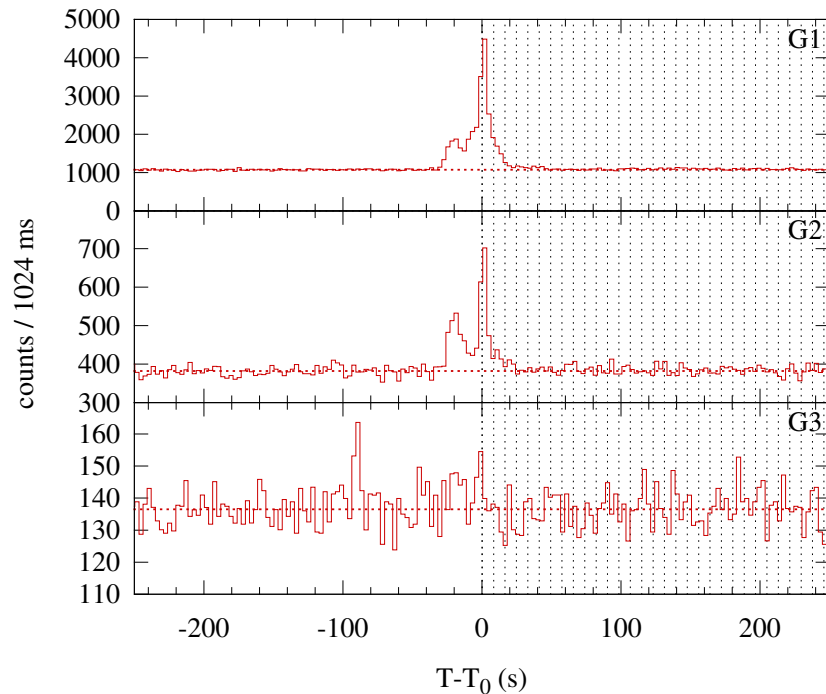
Konus-WIND S2 SOL2014-10-21T10:48 (C6.3) T_0 = 38931.702 s UT (10:48:51.702)
