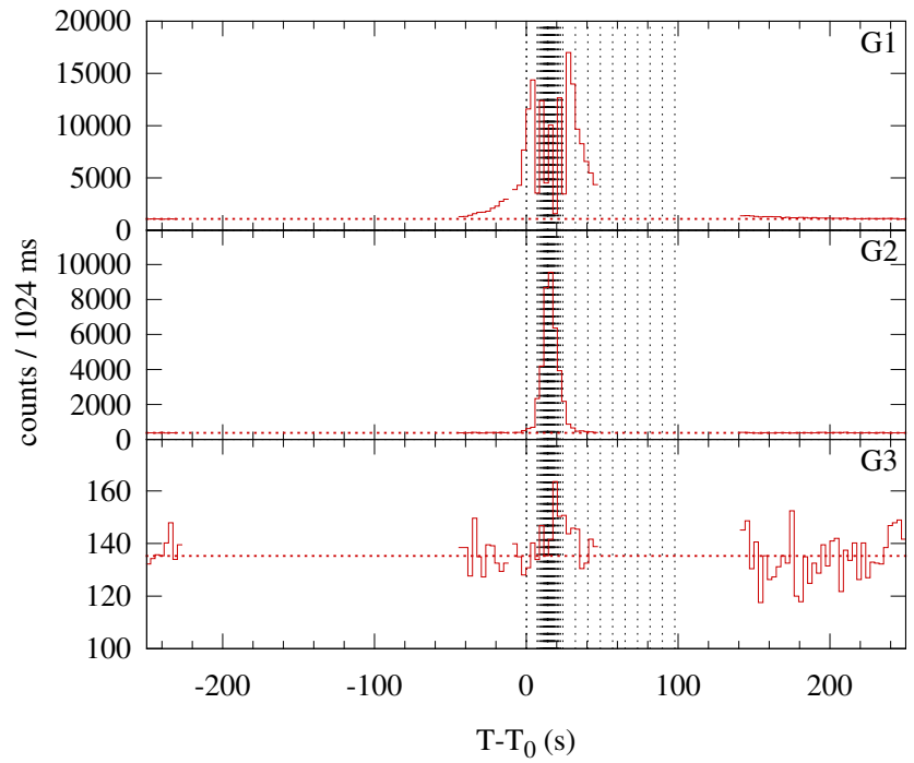
Konus-WIND S2 SOL2014-10-22T05:14 (M2.7) T 0 = 18848.967 s UT (05:14:08.967)
