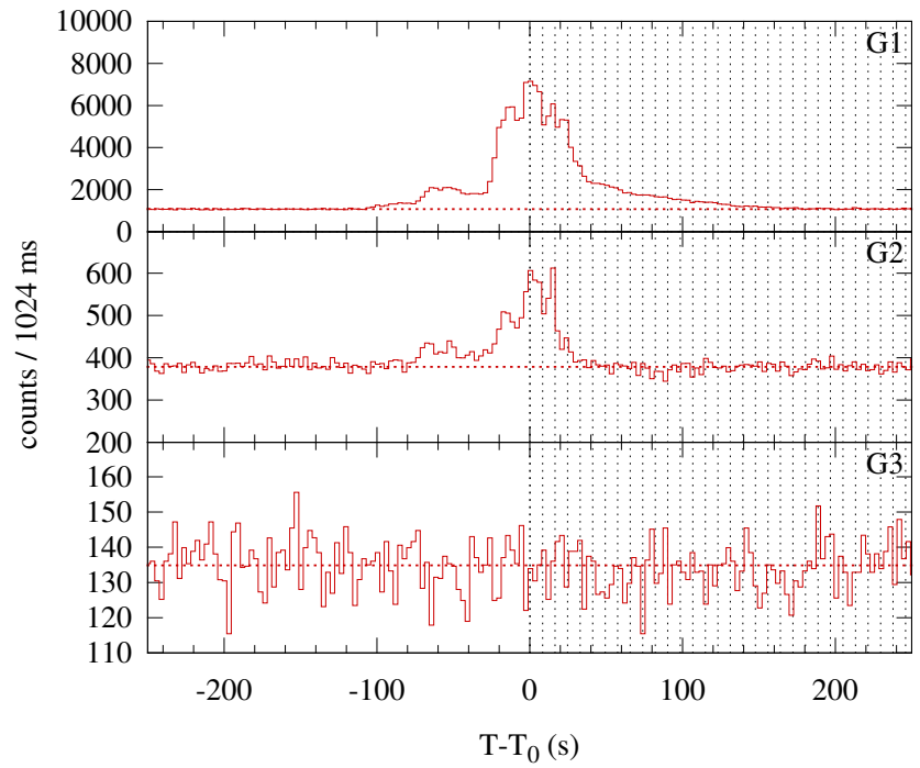
Konus-WIND S2 SOL2014-10-23T09:47 (M1.1) T_0 = 35242.522 s UT (09:47:22.522)
