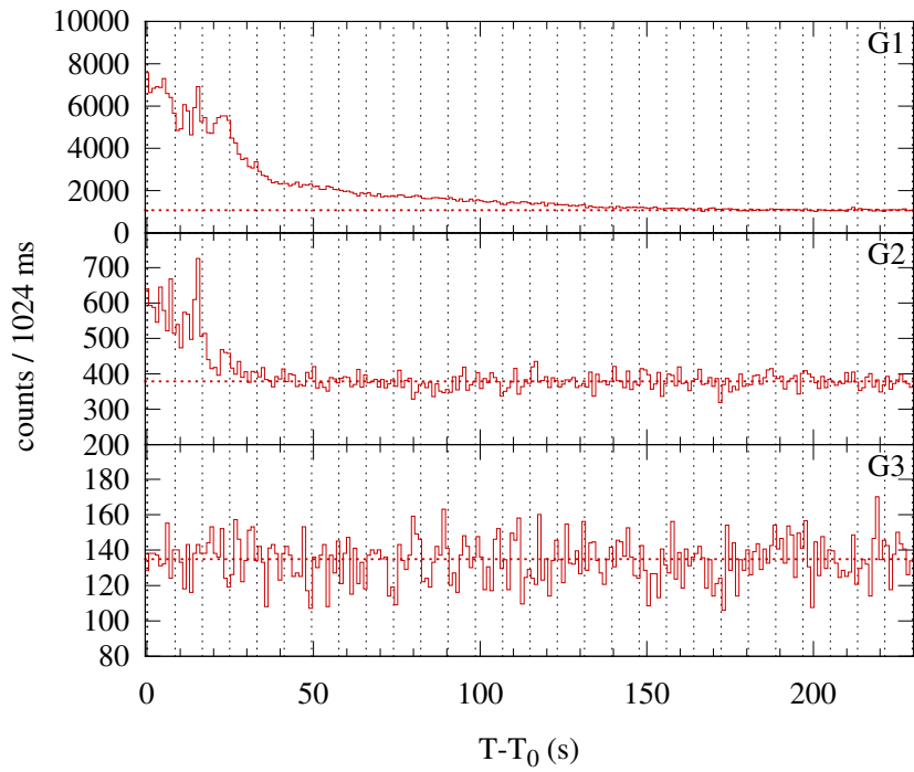
Konus-WIND S2 SOL2014-10-23T09:47 (M1.1) T_0 = 35242.522 s UT (09:47:22.522)
