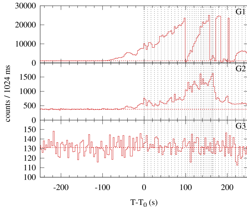
Konus-WIND S2 SOL2014-10-24T21:10 (X3.1) T_0 = 76214.879 s UT (21:10:14.879)
