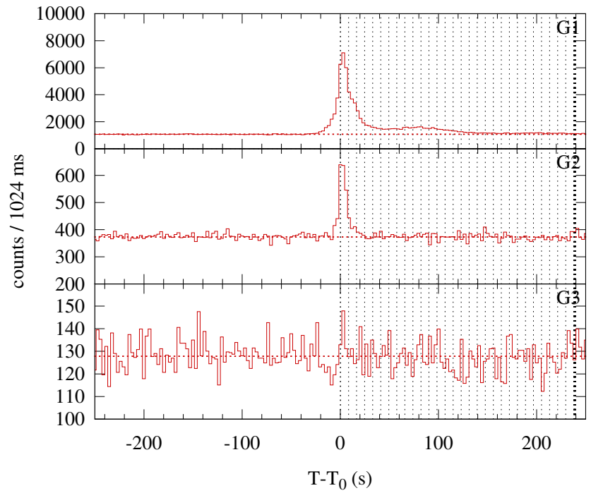
Konus-WIND S2 SOL2014-10-25T23:21 (C8.4) T 0 = 84117.290 s UT (23:21:57.290)
