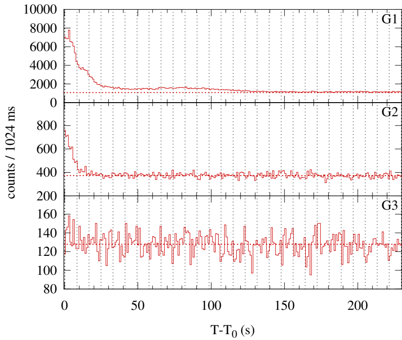
Konus-WIND S2 SOL2014-10-25T23:21 (C8.4) T 0 = 84117.290 s UT (23:21:57.290)
