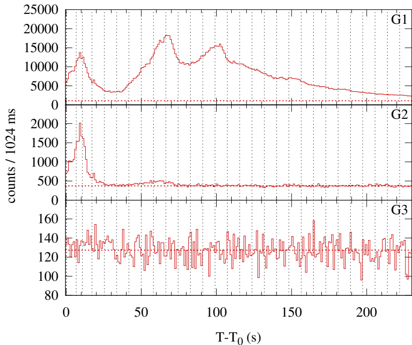
Konus-WIND S2 SOL2014-10-26T18:08 (M4.2) T_0 = 65299.268 s UT (18:08:19.268)
