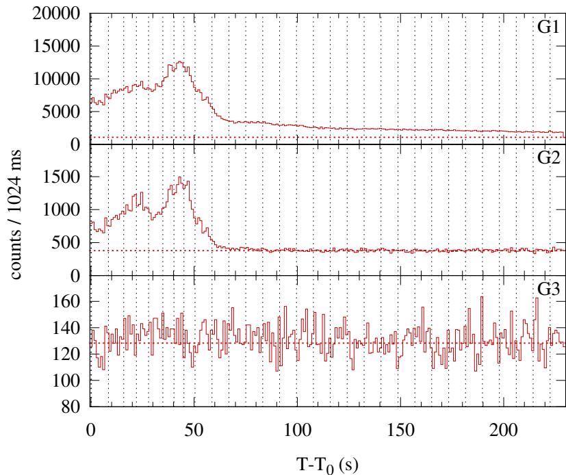
Konus-WIND S2 SOL2014-11-16T17:44 (M5.7) T 0 = 63855.35 s UT (17:44:15.35)
