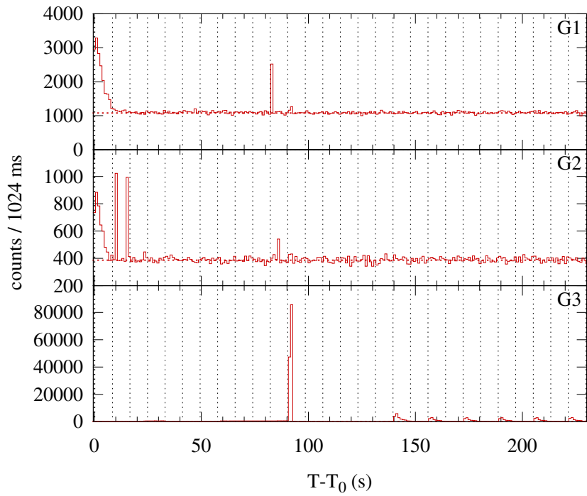
Konus-WIND S2 SOL2014-11-19T21:49 (C2.6) T 0 = 78585.589 s UT (21:49:45.589)
