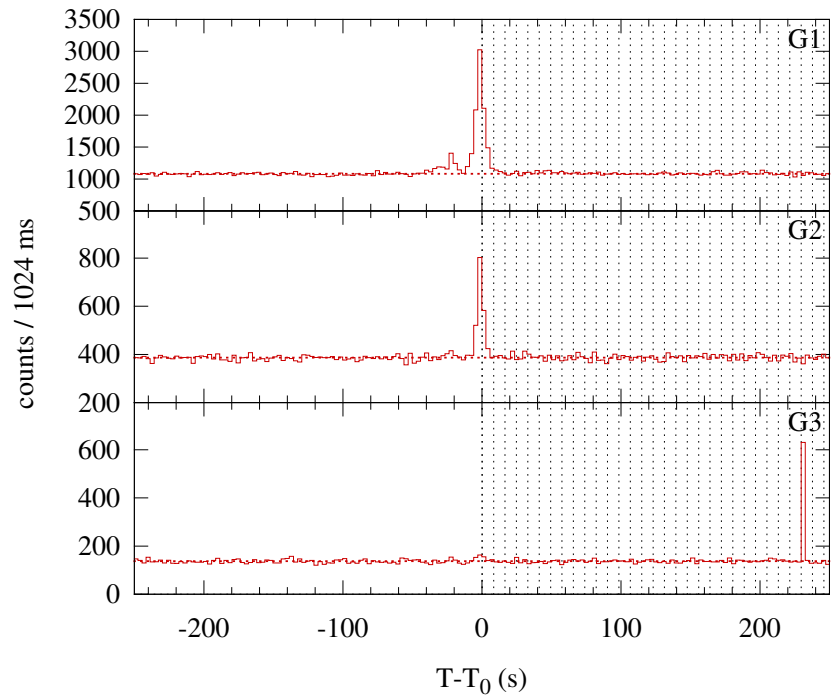
Konus-WIND S2 SOL2014-11-19T21:49 (C2.6) T 0 = 78585.589 s UT (21:49:45.589)
