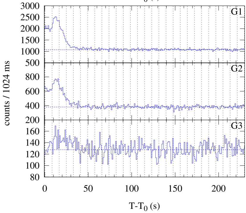
Konus-WIND S2 SOL2014-12-13T10:07 (C4.0) T_0 = 36427.542 s UT (10:07:07.542)
