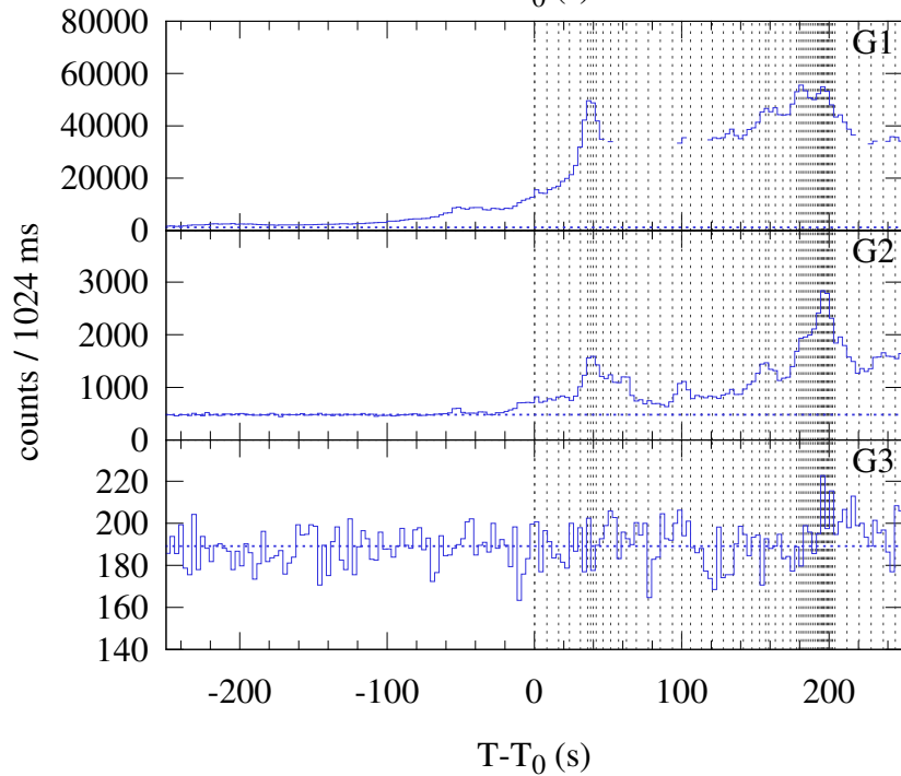
Konus-WIND S2 SOL2014-12-20T00:18 (X1.8) T_0 = 1114.784 s UT (00:18:34.784)
