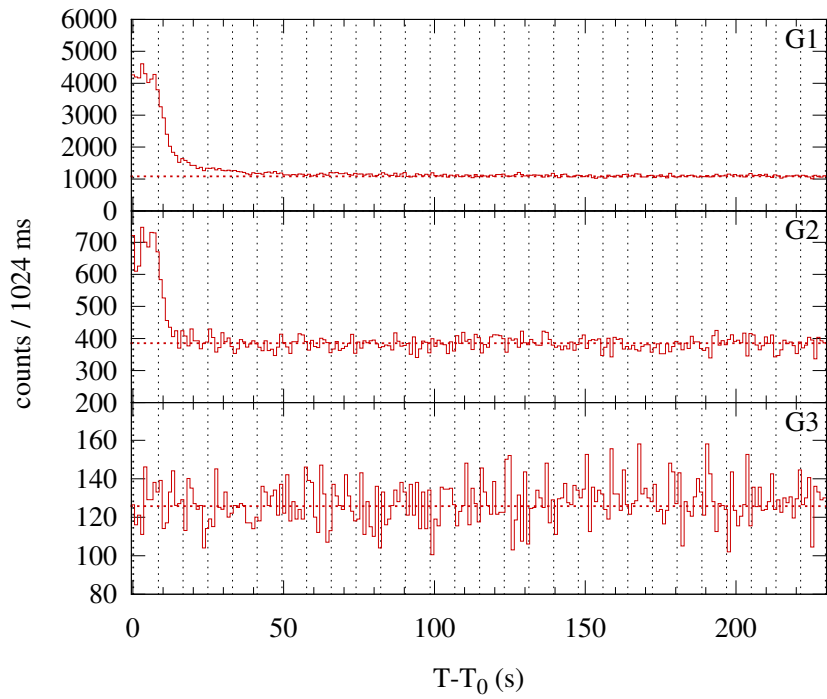
Konus-WIND S2 SOL2015-03-09T10:05 (C4.0) T 0 = 36342.377 s UT (10:05:42.377)
