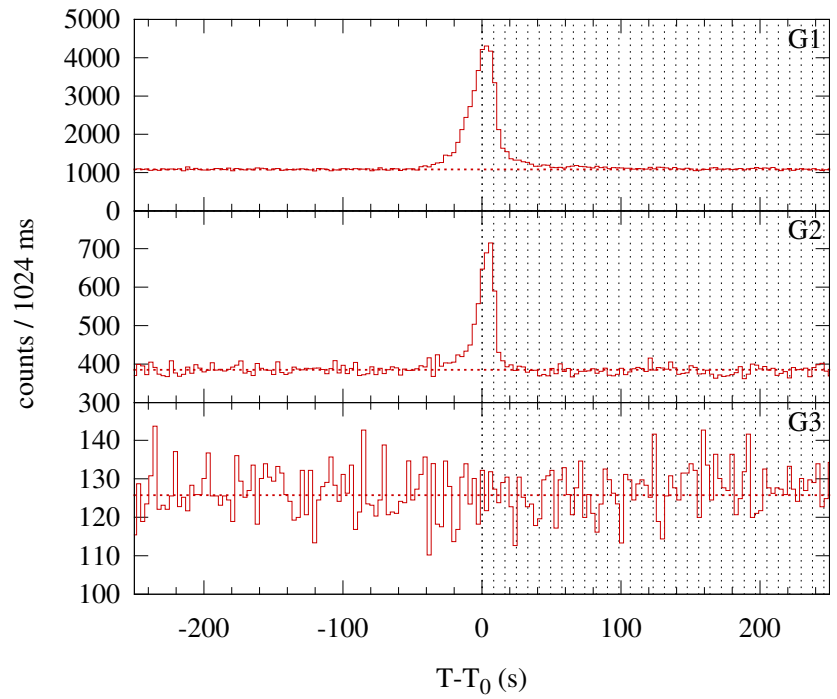
Konus-WIND S2 SOL2015-03-09T10:05 (C4.0) T 0 = 36342.377 s UT (10:05:42.377)
