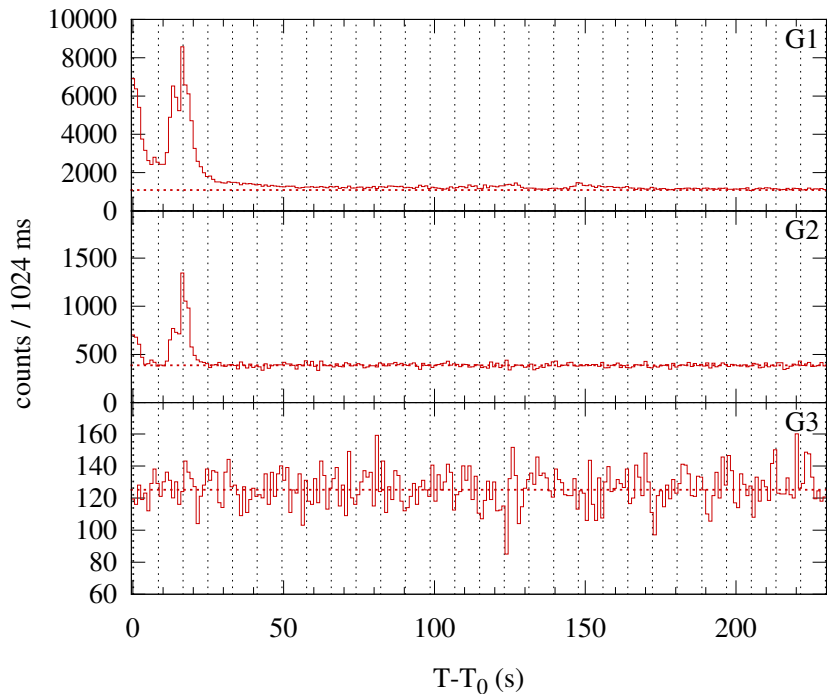
Konus-WIND S2 SOL2015-03-09T17:40 (C9.1) T 0 = 63618.225 s UT (17:40:18.225)
