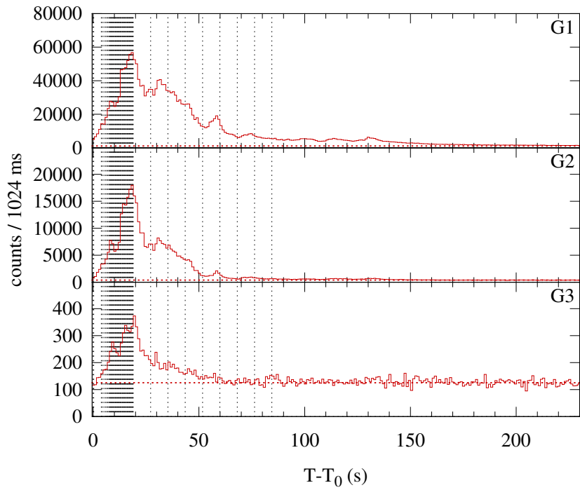
Konus-WIND S2 SOL2015-03-10T03:20 (M5.1) T_0 = 12045.155 s UT (03:20:45.155)
