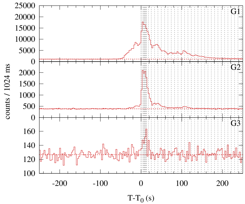
Konus-WIND S2 SOL2015-03-12T04:43 (M3.2) T 0 = 16992.5 s UT (04:43:12.5)
