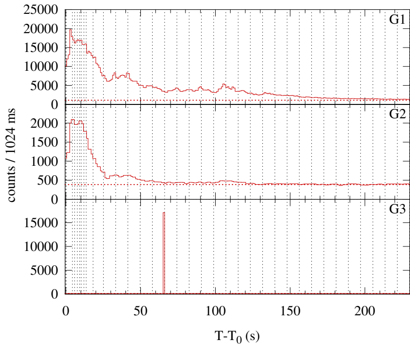
Konus-WIND S2 SOL2015-03-12T04:43 (M3.2) T 0 = 16992.5 s UT (04:43:12.5)
