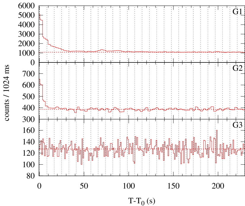
Konus-WIND S2 SOL2015-06-18T00:22 (C7.2) T 0 = 1339.768 s UT (00:22:19.768)
