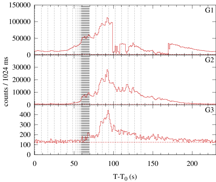
Konus-WIND S2 SOL2015-06-25T08:12 (M7.9) T_0 = 29571.248 s UT (08:12:51.248)
