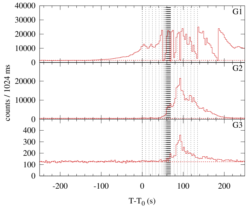
Konus-WIND S2 SOL2015-06-25T08:12 (M7.9) T_0 = 29571.248 s UT (08:12:51.248)
