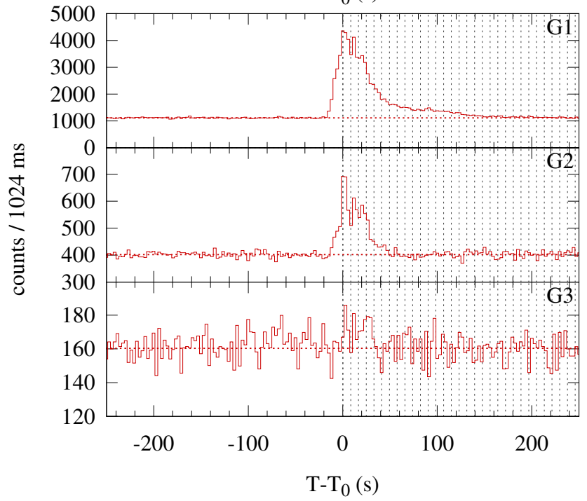
Konus-WIND S2 SOL2017-07-03T16:13 (M1.3) T_0 = 58402.622 s UT (16:13:22.622)
