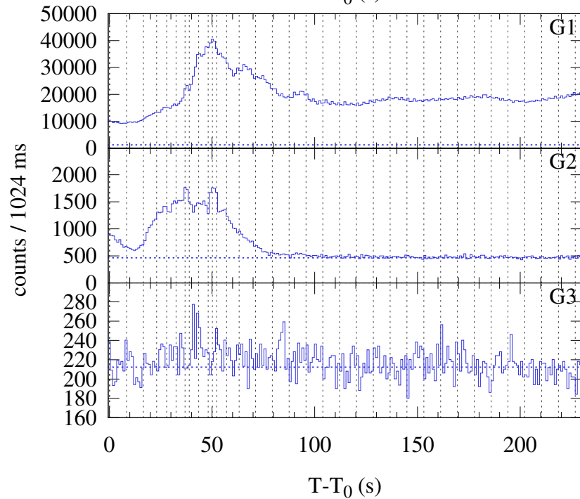
Konus-WIND S2 SOL2017-09-06T09:03 (X2.2) T 0 = 32582.225 s UT (09:03:02.225)
