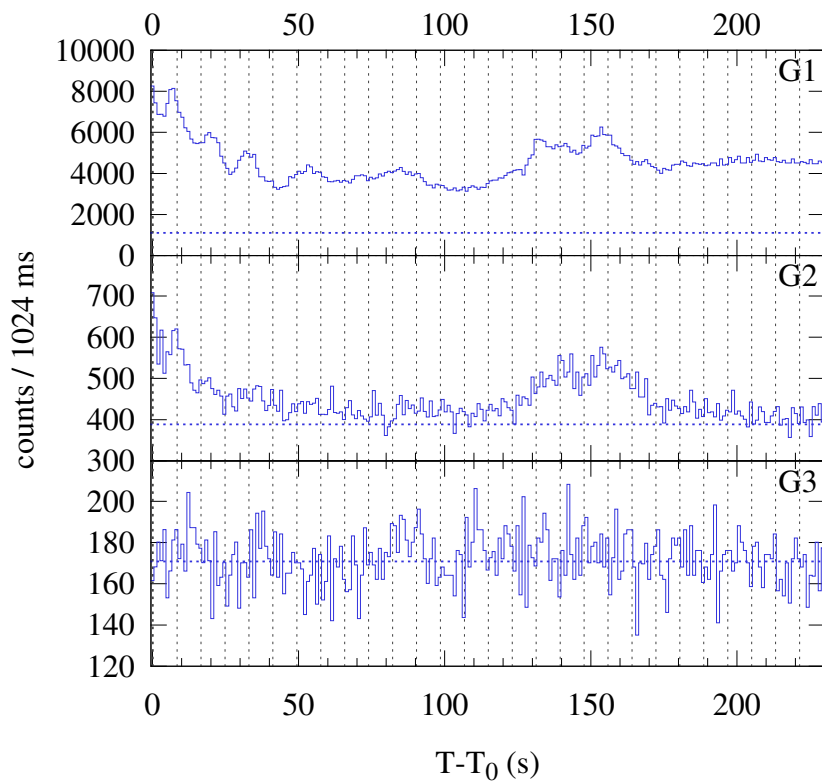
Konus-WIND S2 SOL2022-03-30T17:31 (X1.3) T_0 = 63066.179 s UT (17:31:06.179)
