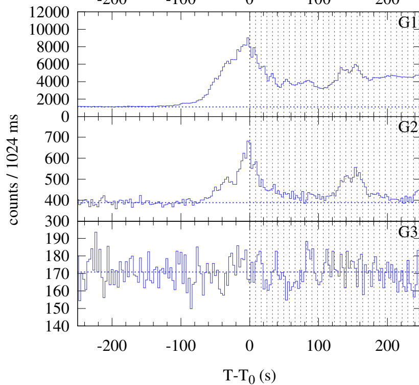
Konus-WIND S2 SOL2022-03-30T17:31 (X1.3) T_0 = 63066.179 s UT (17:31:06.179)
