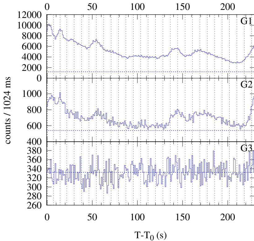
Konus-WIND S2 SOL2022-03-31T18:28 (M9.6) T_0 = 66484.815 s UT (18:28:04.815)
