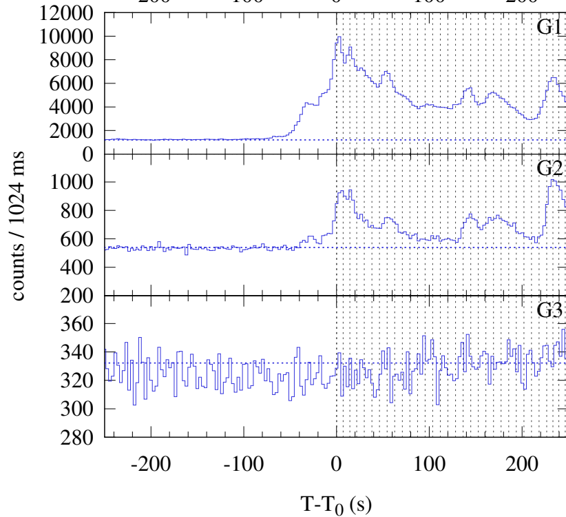
Konus-WIND S2 SOL2022-03-31T18:28 (M9.6) T_0 = 66484.815 s UT (18:28:04.815)
