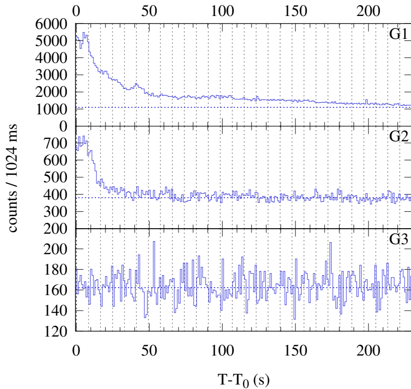
Konus-WIND S2 SOL2022-04-17T22:32 (M4.4) T_0 = 81140.248 s UT (22:32:20.248)
