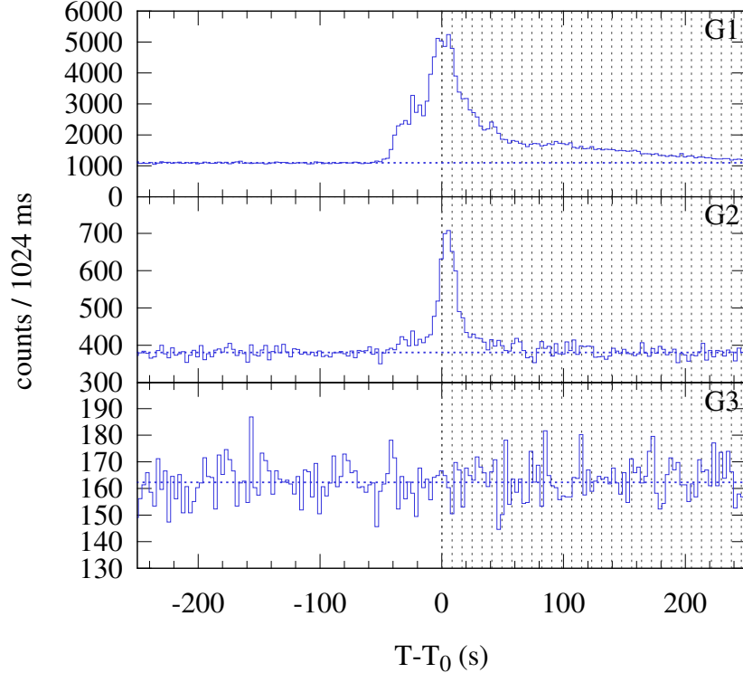
Konus-WIND S2 SOL2022-04-17T22:32 (M4.4) T_0 = 81140.248 s UT (22:32:20.248)
