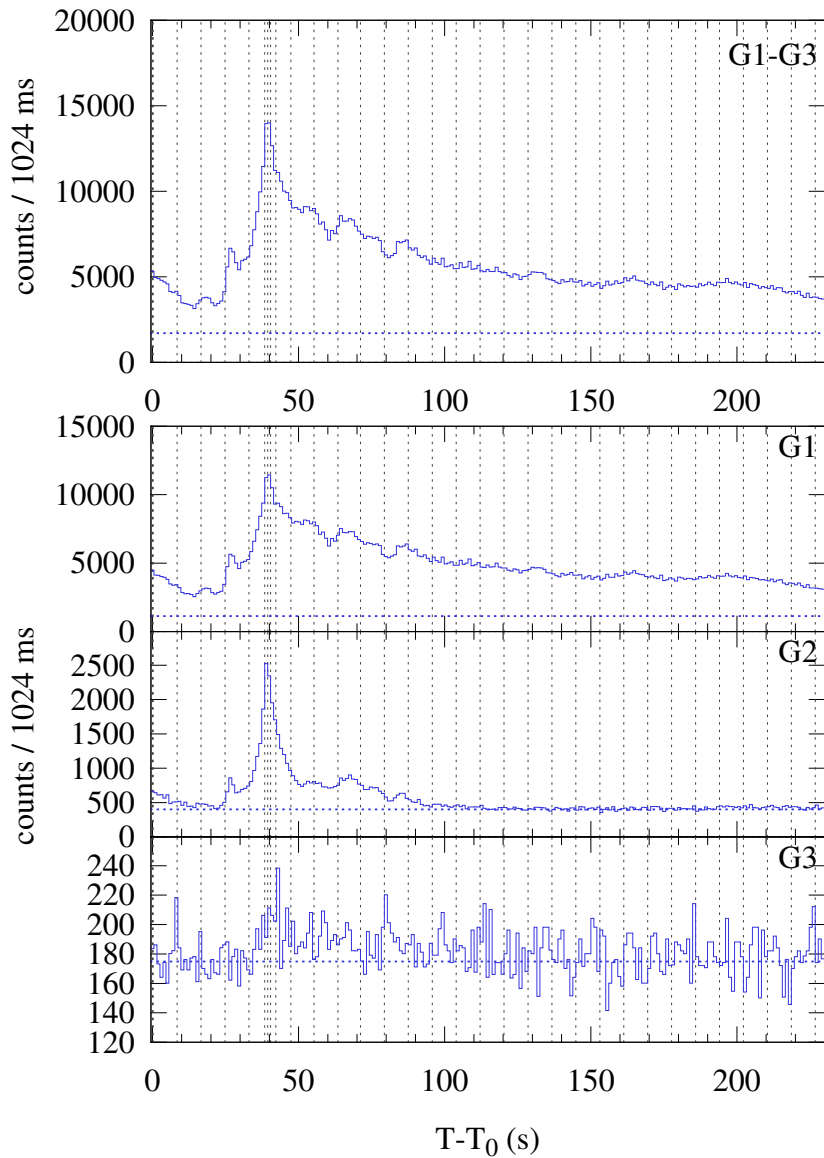
Konus-WIND S2 SOL2022-04-30T13:42 (X1.1) T_0 = 49362.134 s UT (13:42:42.134)
