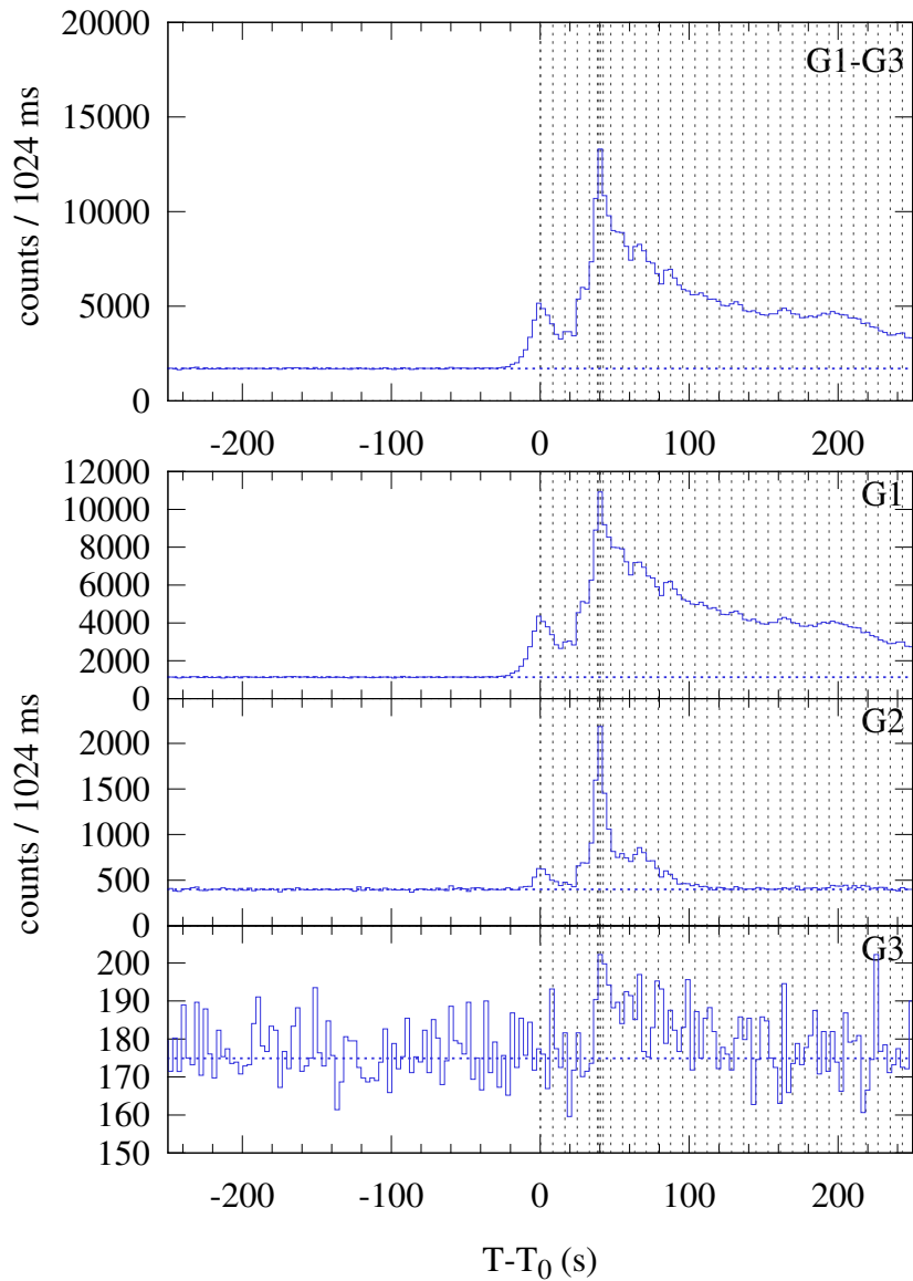
Konus-WIND S2 SOL2022-04-30T13:42 (X1.1) T_0 = 49362.134 s UT (13:42:42.134)
